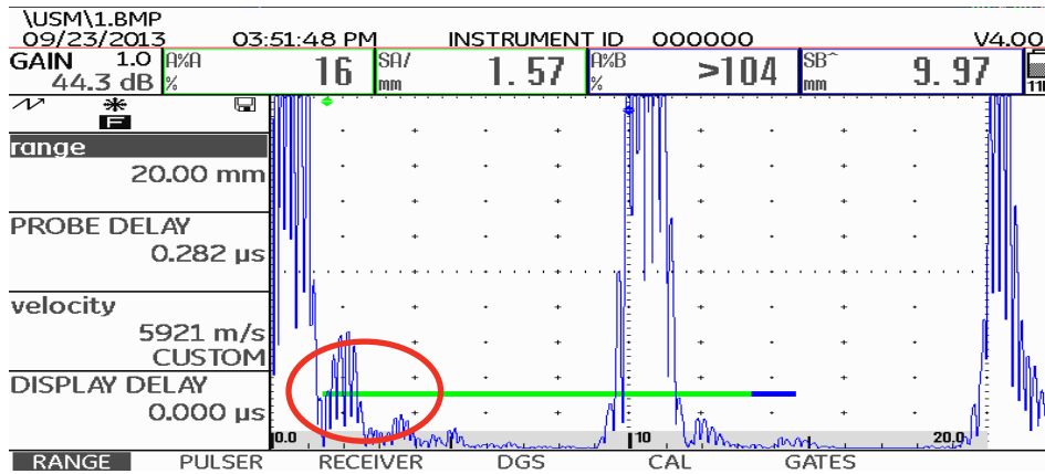
1.6 mm FBH with USM 36
