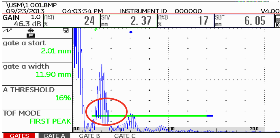
2.3 mm Corrosion with USM 36
